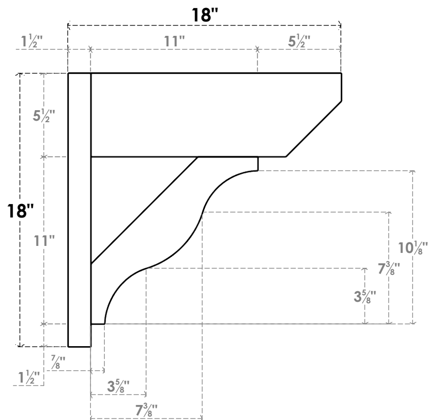
SIDE PROFILE
